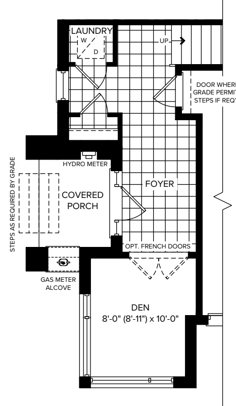
PARTIAL GROUND FLOOR ELEVATION A2
