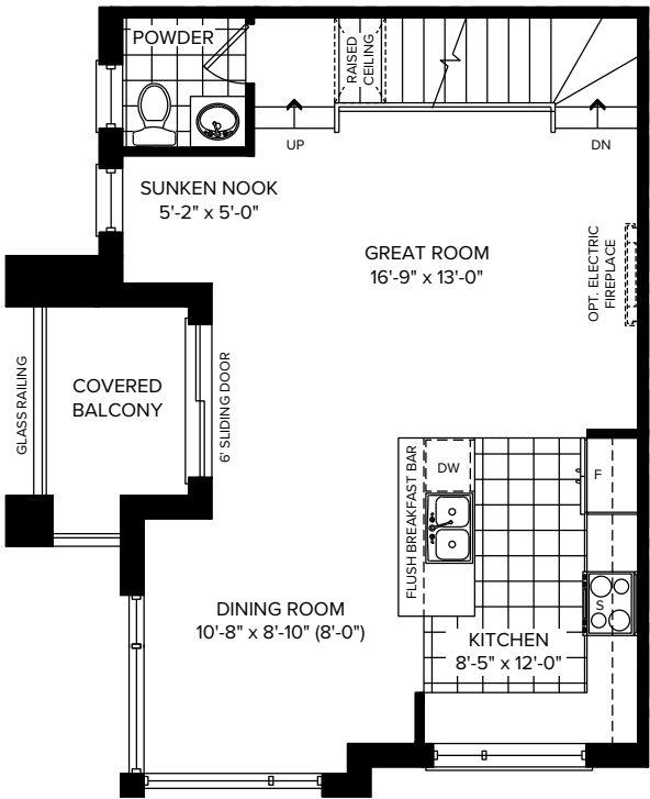
MAIN FLOOR ELEVATION A1
