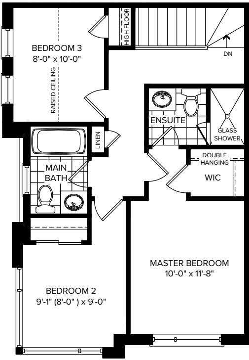
THIRD FLOOR ELEVATION A1
