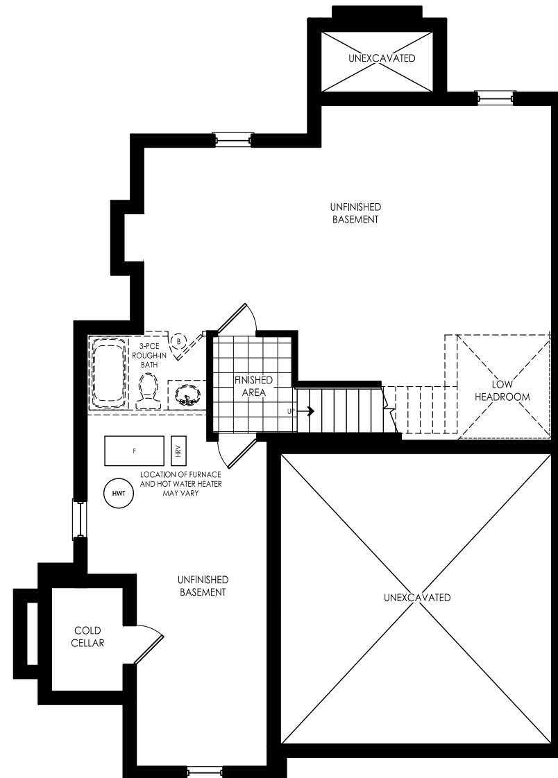
BASEMENT A
