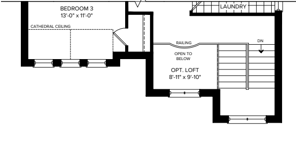
PARTIAL SECOND FLOOR ELEVATION B
