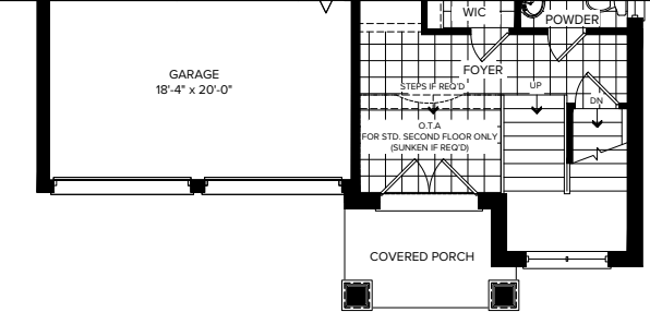
PARTIAL GROUND FLOOR ELEVATION B
