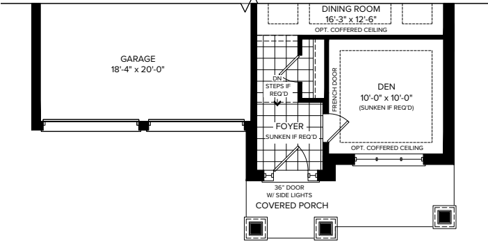
PARTIAL GROUND FLOOR ELEVATION C
