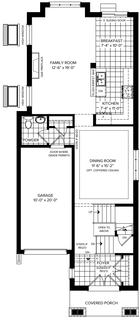
PARTIAL GROUND FLOOR ELEVATION C
