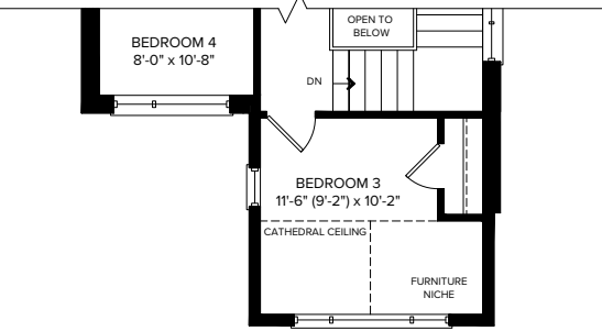
PARTIAL SECOND FLOOR ELEVATION C
