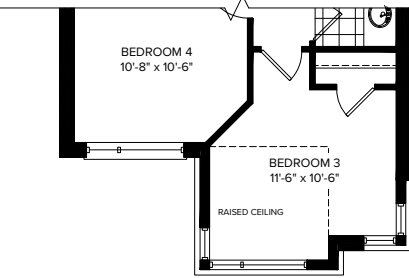
PARTIAL SECOND FLOOR ELEVATION C
