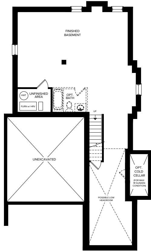
FINISHED BASEMENT ELEVATION A
