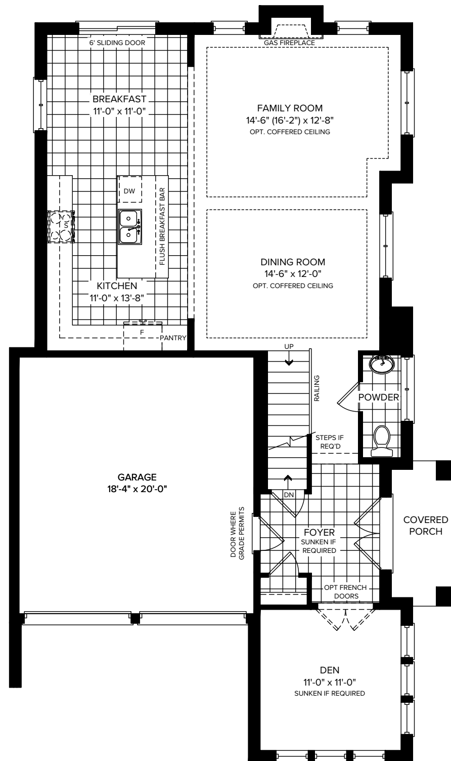
GROUND FLOOR ELEVATION B
