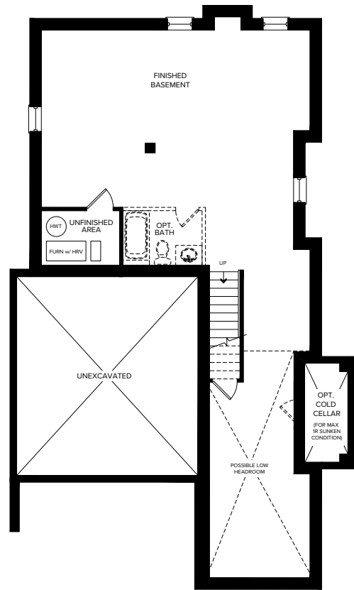
FINISHED BASEMENT ELEVATION B
