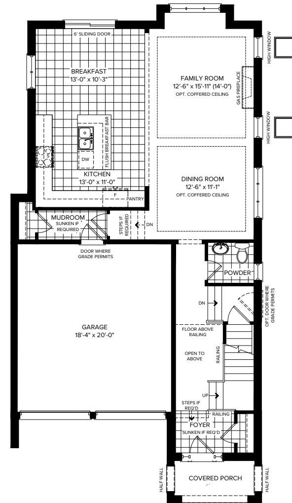
PARTIAL GROUND FLOOR ELEVATION B
