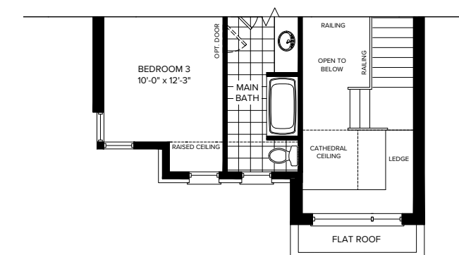
PARTIAL SECOND FLOOR ELEVATION C
