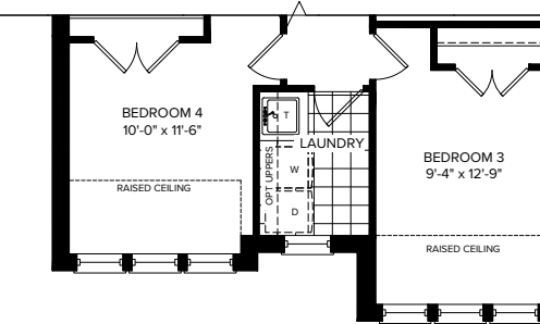
PARTIAL SECOND FLOOR ELEVATION B
