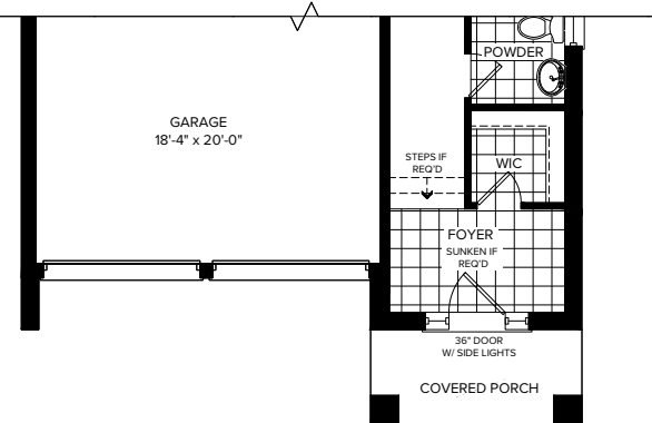
PARTIAL GROUND FLOOR ELEVATION C
