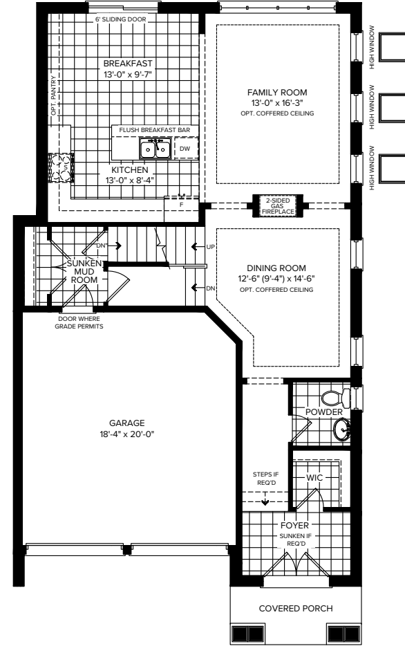
PARTIAL GROUND FLOOR ELEVATION B
