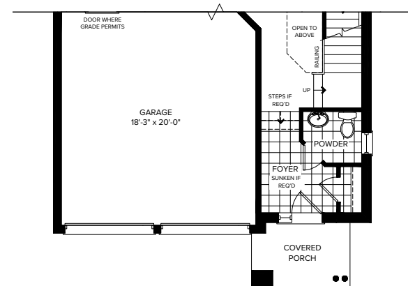
PARTIAL GROUND FLOOR ELEVATION C
