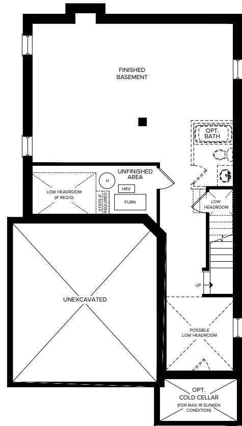
PARTIAL FINISHED BASEMENT ELEVATION C
