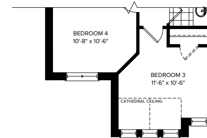
PARTIAL SECOND FLOOR ELEVATION B
