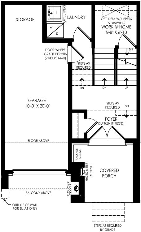
GROUND FLOOR ELEV. A
