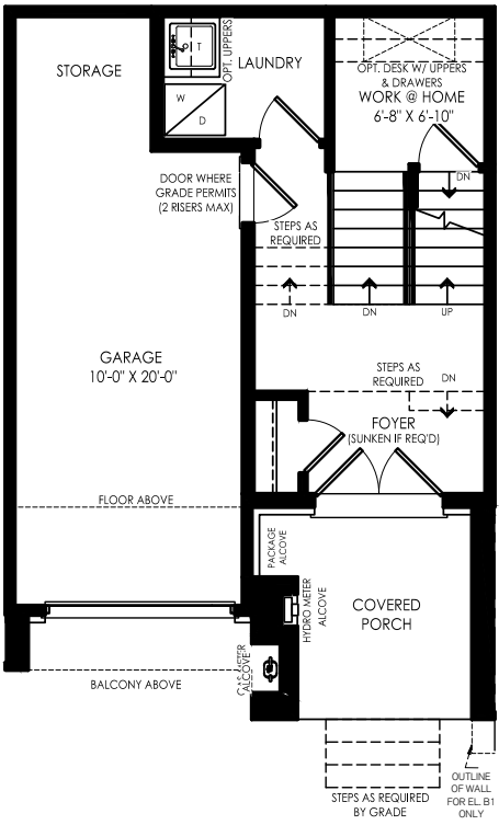
GROUND FLOOR ELEV. B
