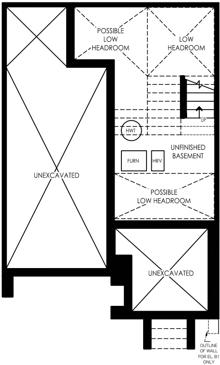
BASEMENT ELEV. B
