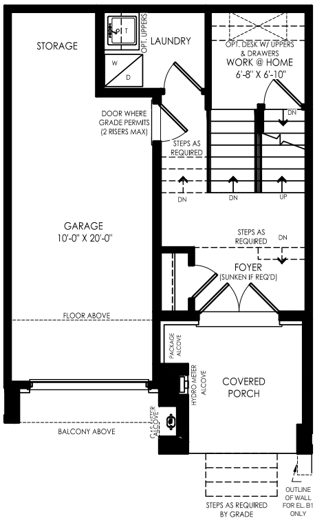
GROUND FLOOR ELEV. B
