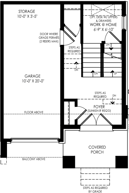
GROUND FLOOR ELEV. B
