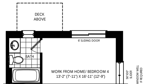
OPT. FINISHED BASEMENT WALK-OUT ELEV. A & B & C
