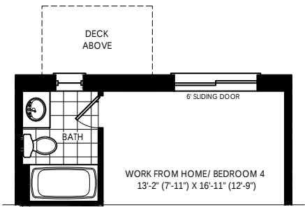
OPT. FINISHED BASEMENT WALK-OUT ELEV. A & B & C
