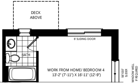
OPT. FINISHED BASEMENT WALK-OUT ELEV. A & B & C
