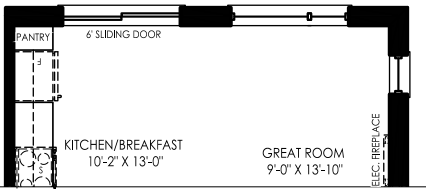
GROUND FLOOR ELEV. C
