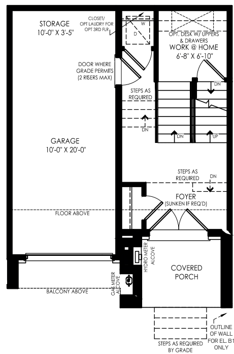
GROUND FLOOR ELEV. B (OPTIONAL 2 BATHROOM)
