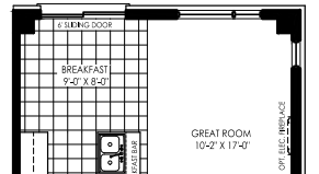
GROUND FLOOR ELEV. B
