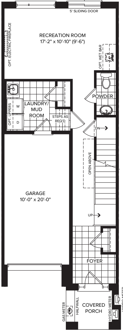
GROUND FLOOR ELEVATION A
