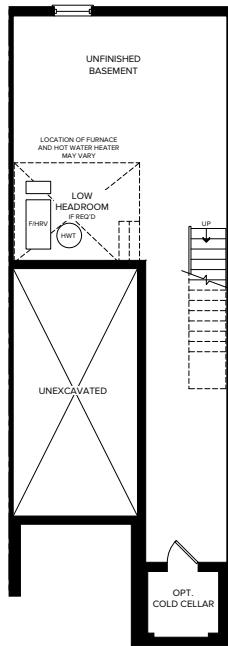
BASEMENT FLOOR
