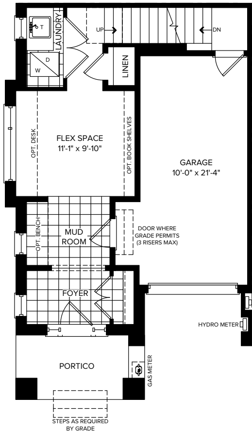
GROUND FLOOR ELEVATION B
