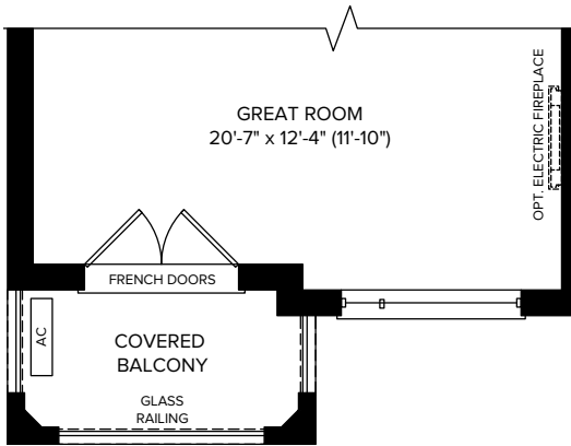
PARTIAL MAIN FLOOR ELEVATION B
