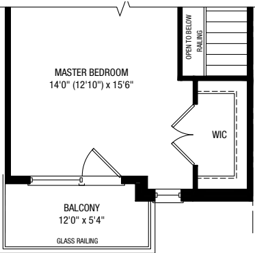
PARTIAL THIRD B
