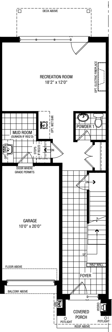
PARTIAL GROUND AND OPT. GROUND B
