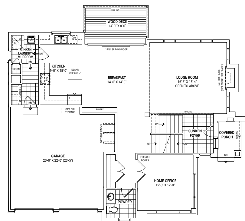
GROUND FLOOR PLAN ELEVATION A
