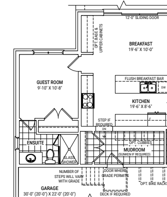
PARTIAL GROUND FLOOR PLAN ELE. A & D W/ OPT. GUEST ROOM
