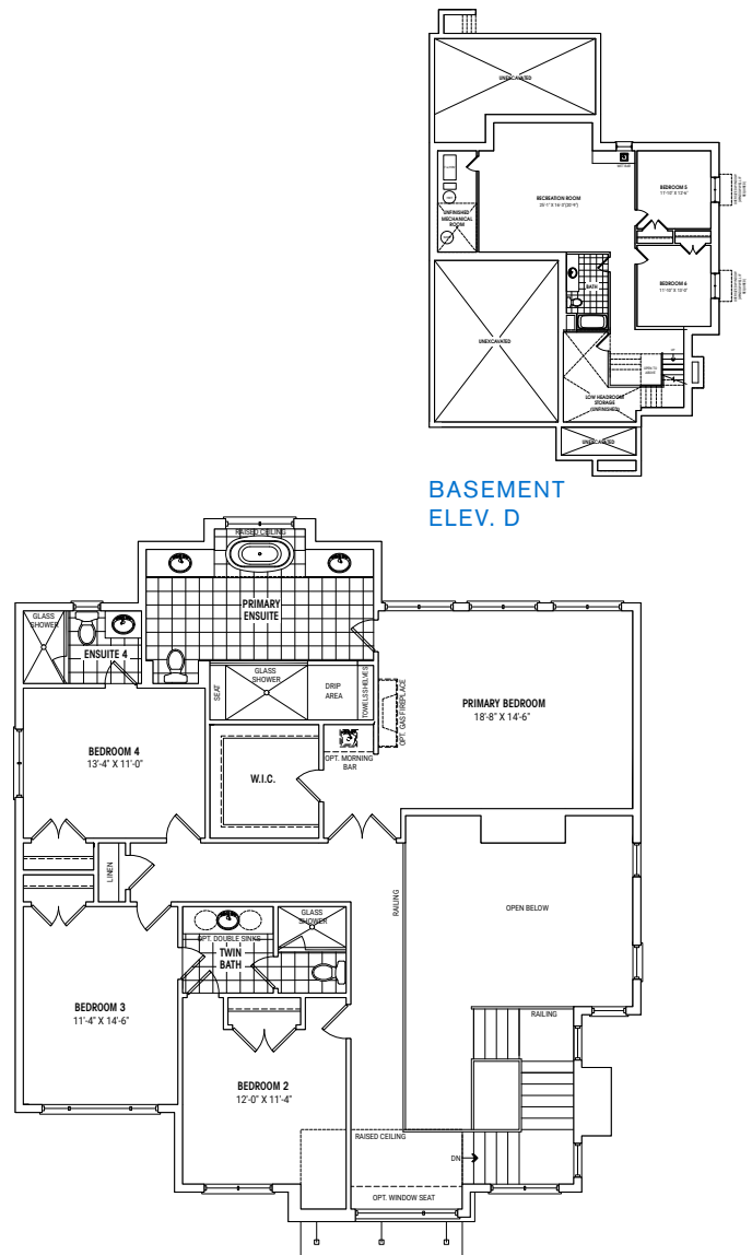
SECOND FLOOR ELEV. D
