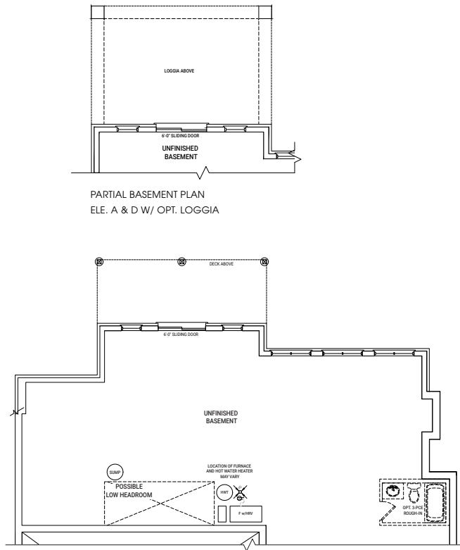
OPT. BASEMENT PLAN WITH GUEST ROOM ELEVATION A
