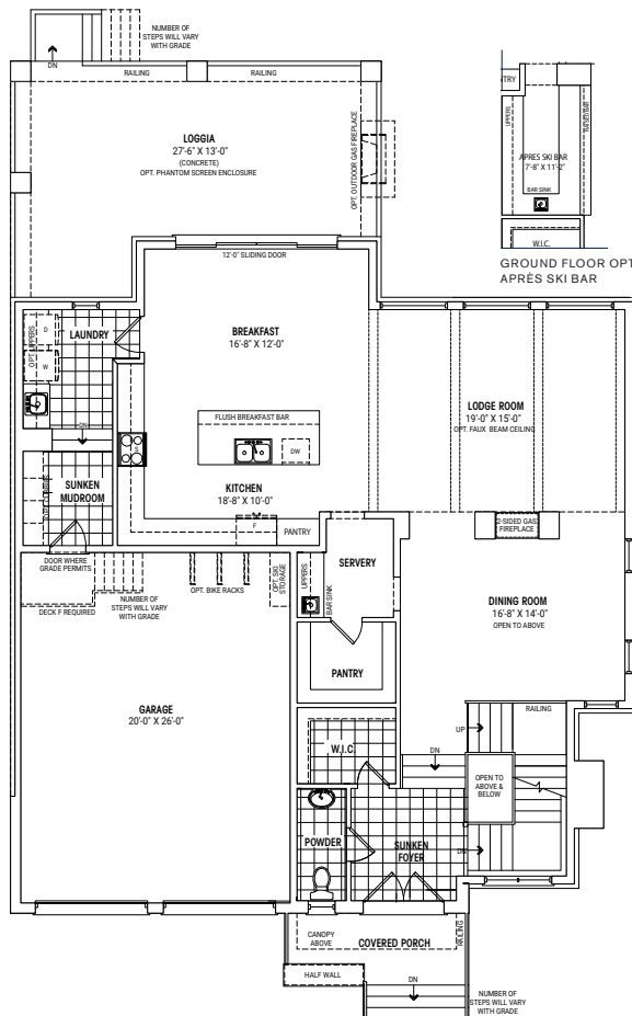
GROUND FLOOR ELEV. D
