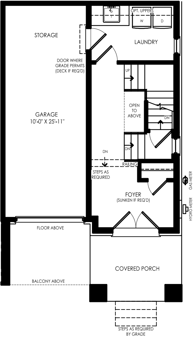
GROUND FLOOR ELEV. A & B
