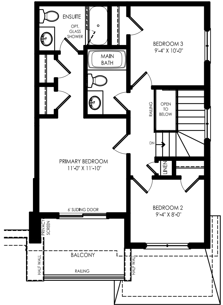
THIRD FLOOR ELEV. A
