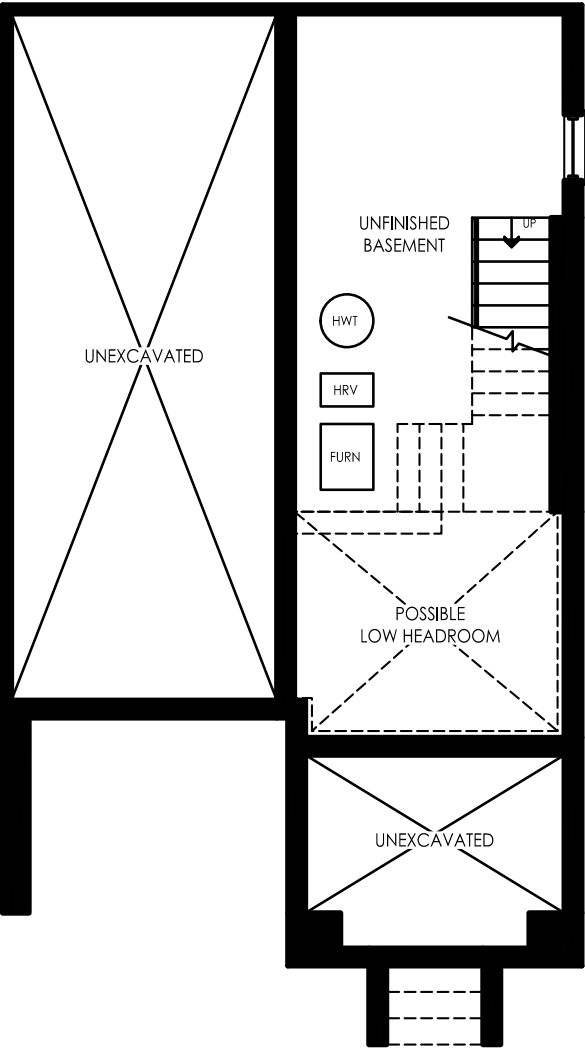
BASEMENT ELEV. A & B
