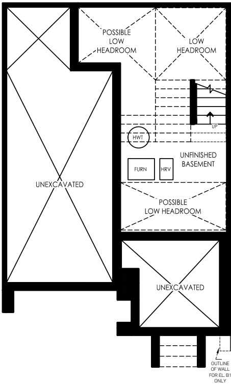
BASEMENT ELEV. B
