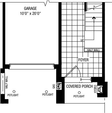
PARTIAL GROUND AND OPT. GROUND B
