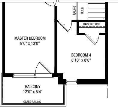
PARTIAL OPTIONAL THIRD B
