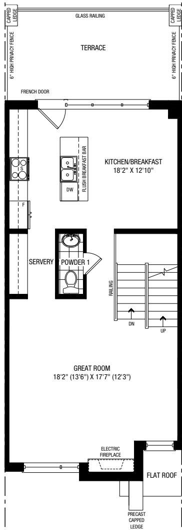
PARTIAL MAIN B PARTIAL MAIN C
