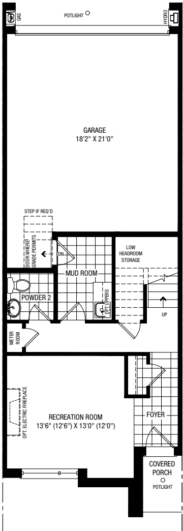
PARTIAL GROUND B PARTIAL GROUND C
