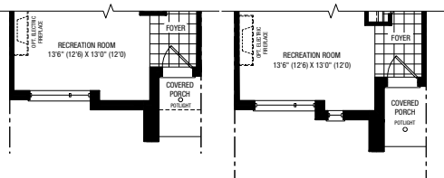
PARTIAL GROUND B PARTIAL GROUND C
