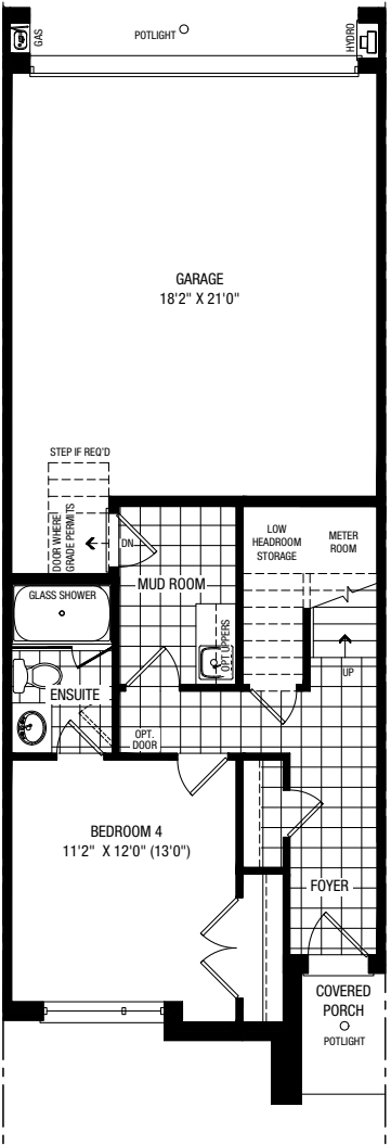
PARTIAL OPT. GROUND B PARTIAL OPT. GROUND C
