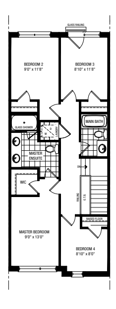
OPT. THIRD A 4 BEDROOM PLAN
