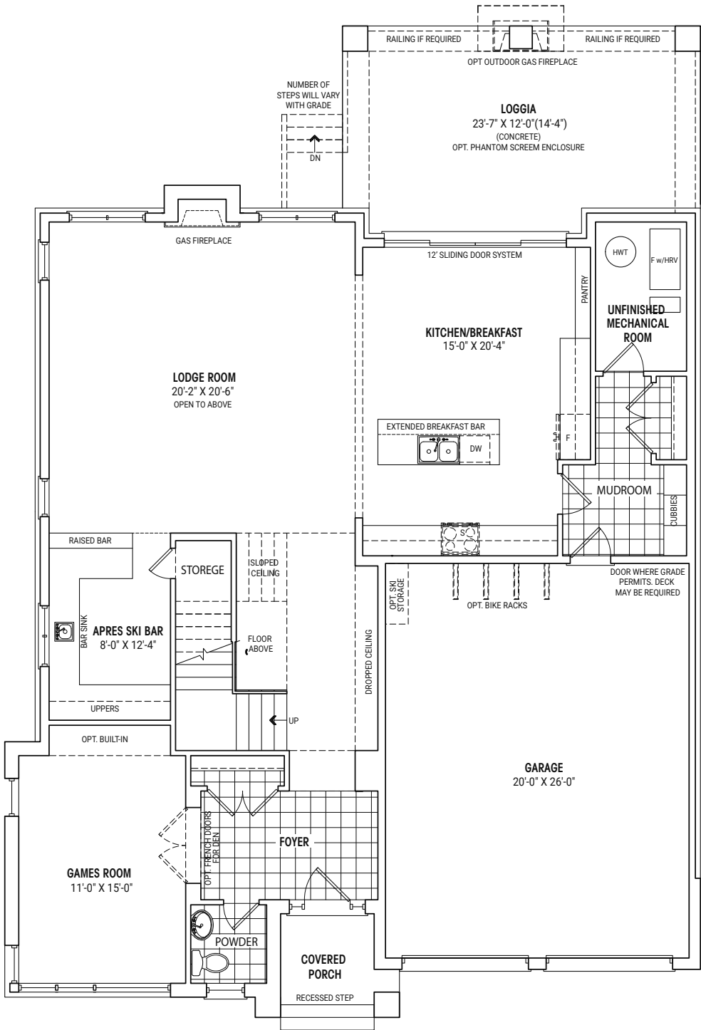
GROUND FLOOR PLAN ELEVATION A
