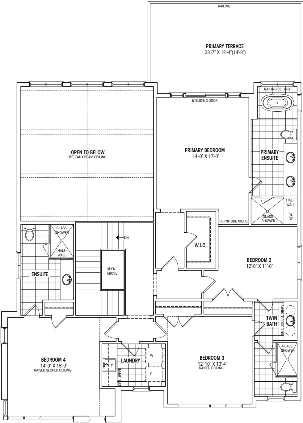
SECOND FLOOR PLAN ELEVATION A
