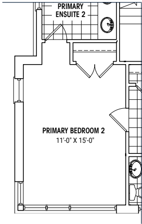
GROUND FLOOR PLAN W/ OPT. 2ND PRIMARY BEDROOM
