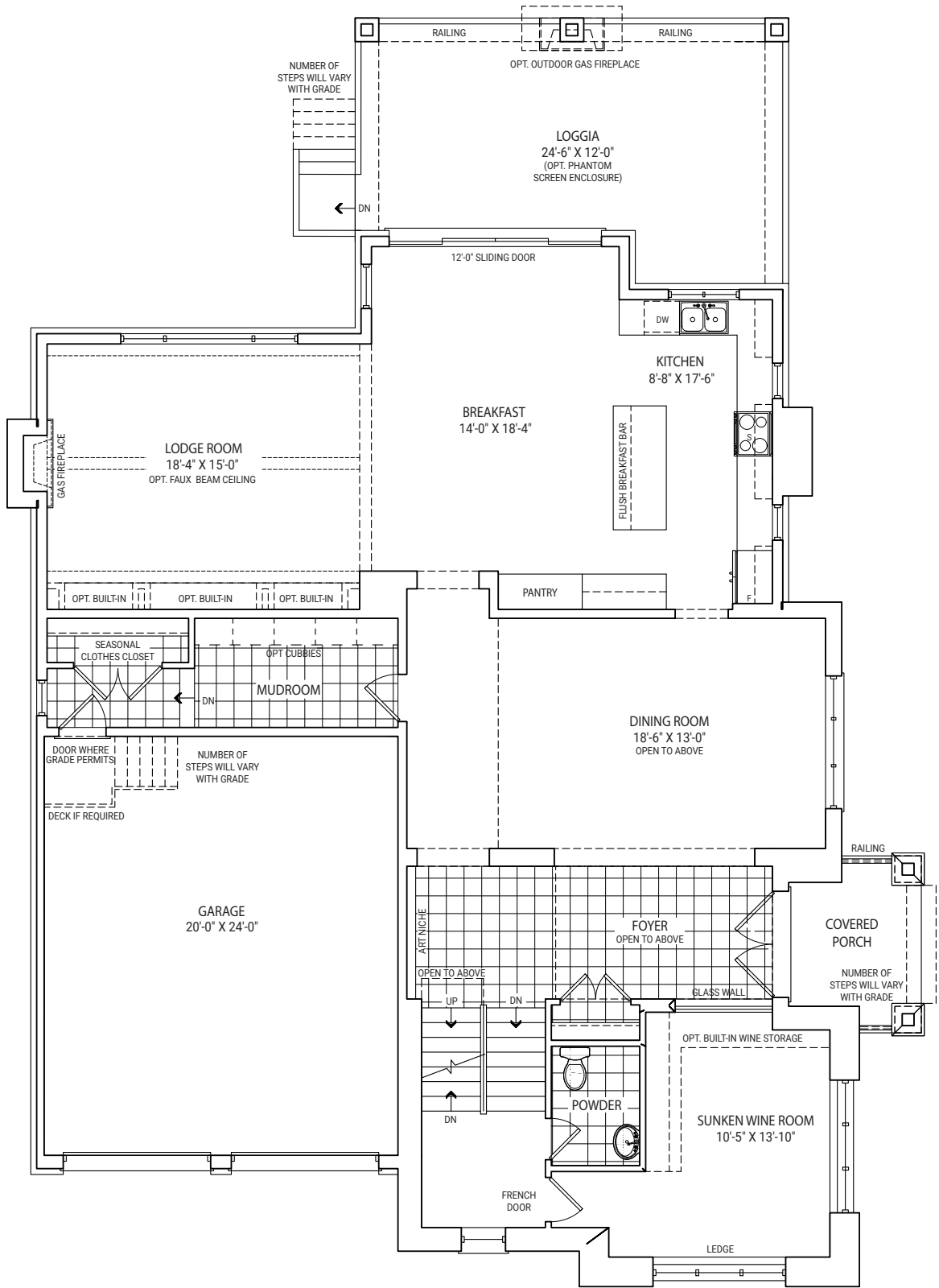
GROUND FLOOR PLAN ELEVATION C
