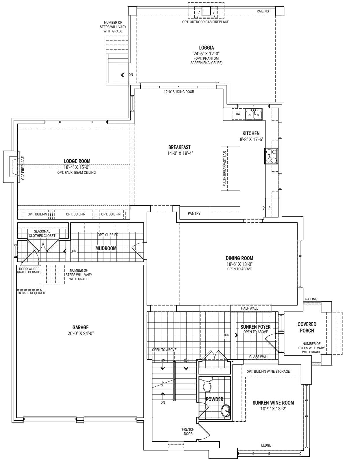
GROUND FLOOR PLAN ELEVATION A
