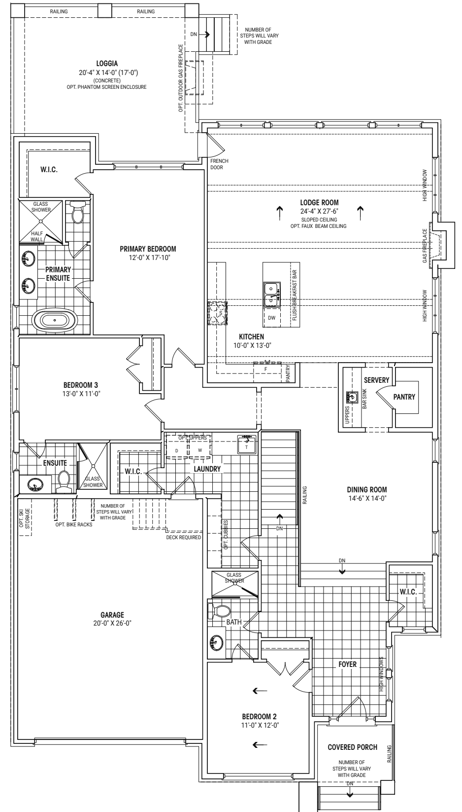
GROUND FLOOR PLAN ELEVATION B
