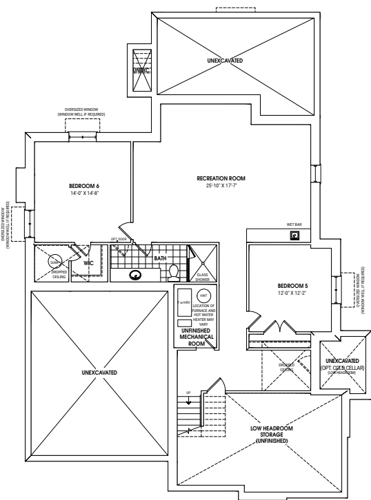
BASEMENT PLAN ELEVATION B
