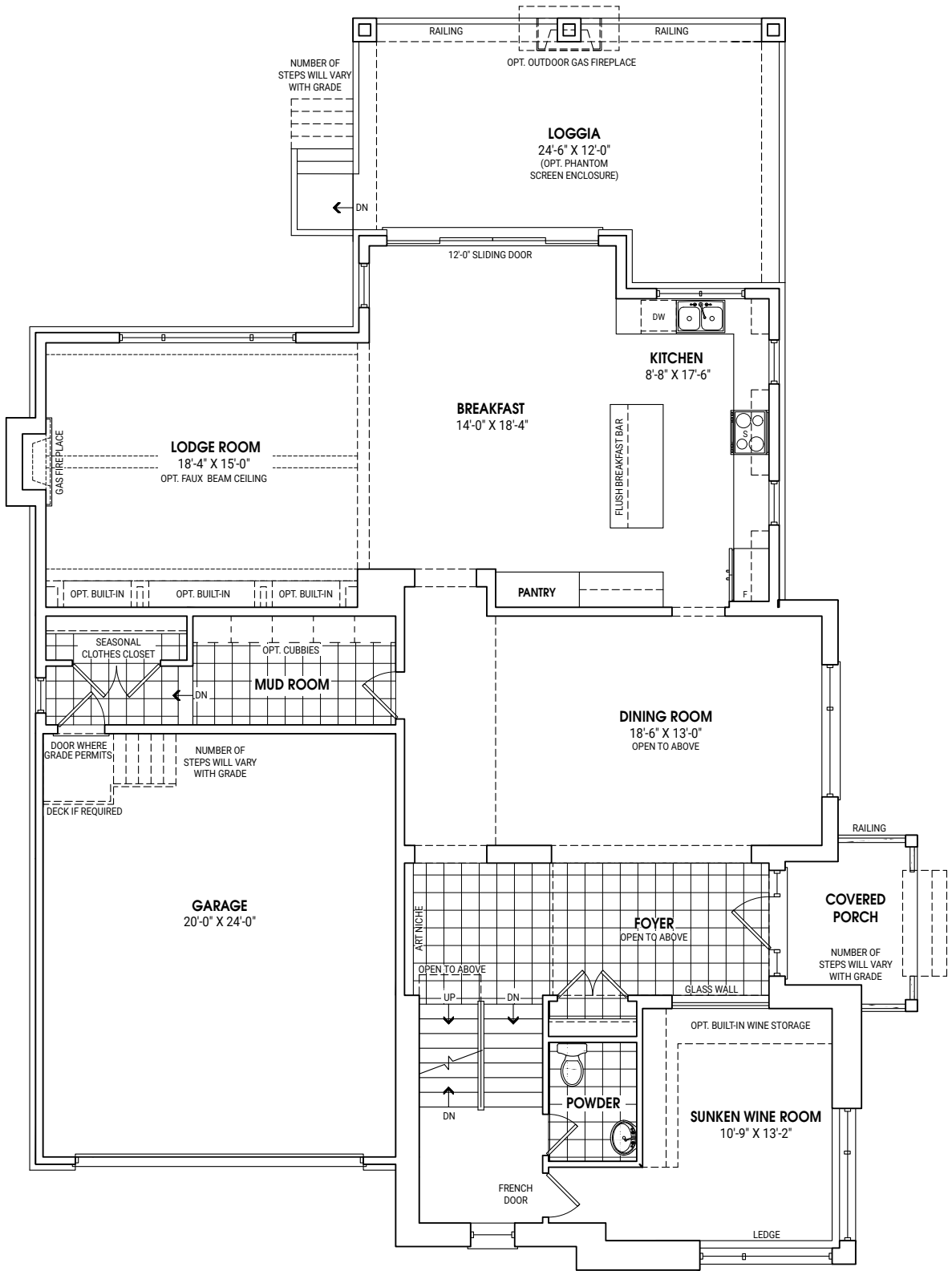
GROUND FLOOR PLAN ELEVATION B
