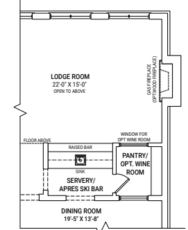
PARTIAL GROUND FLOOR PLAN ELEV. A & D W/ OPT. APRES SKI BAR & OPT. WINE ROOM
