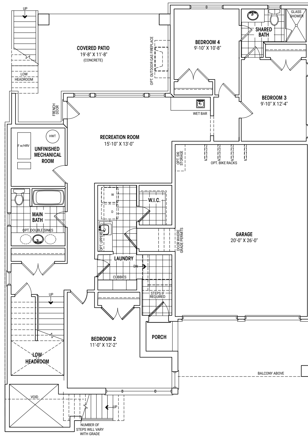
GROUND FLOOR PLAN ELEVATION D
