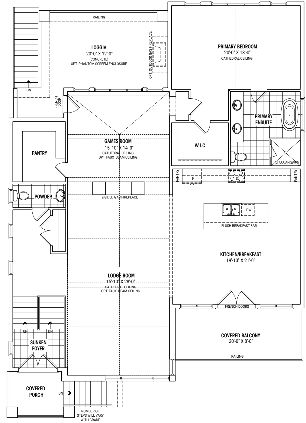
SECOND FLOOR PLAN ELEVATION D
