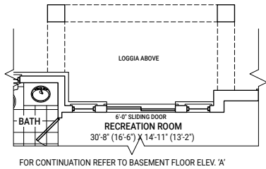
OPT. FINISHED BASEMENT PLAN ELEVATION A W/ OPT. LOGGIA
