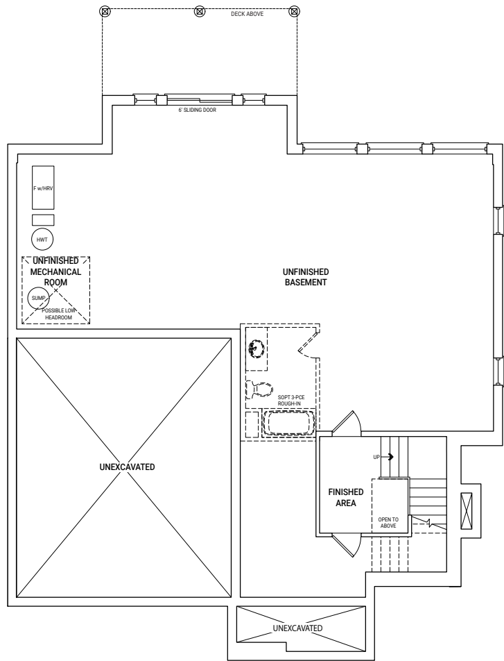
BASEMENT PLAN ELEVATION D
