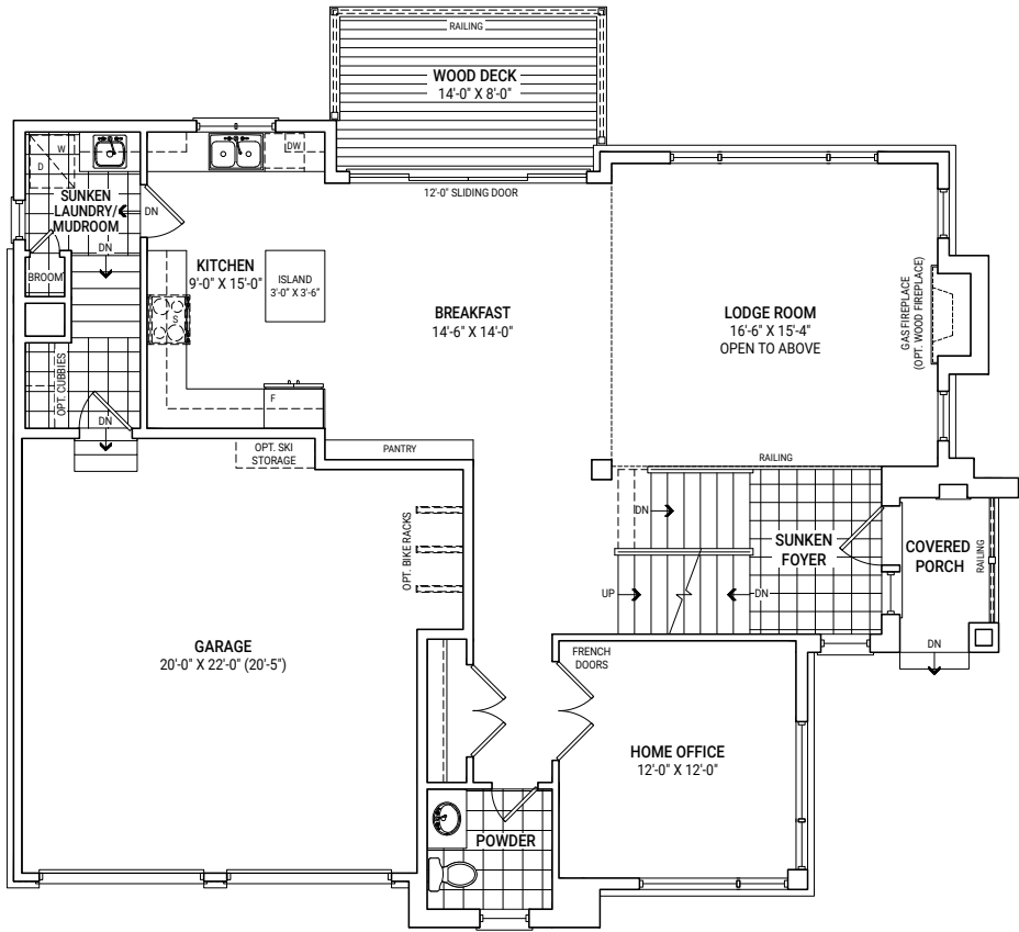
GROUND FLOOR PLAN ELEVATION A
