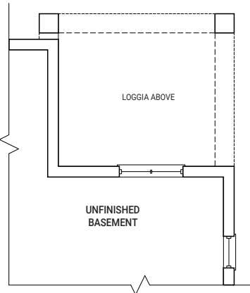
PARTIAL OPT. BASEMENT PLAN W/ OPT. LOGGIA
