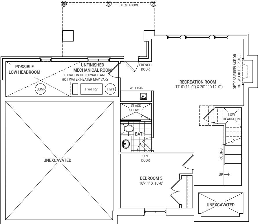
OPT. FINISHED BASEMENT PLAN ELEVATION A
