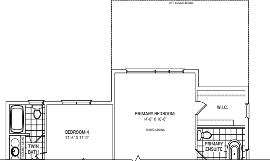
PARTIAL SECOND FLOOR PLAN ELEVATION A W/ OPT. LOGGIA
