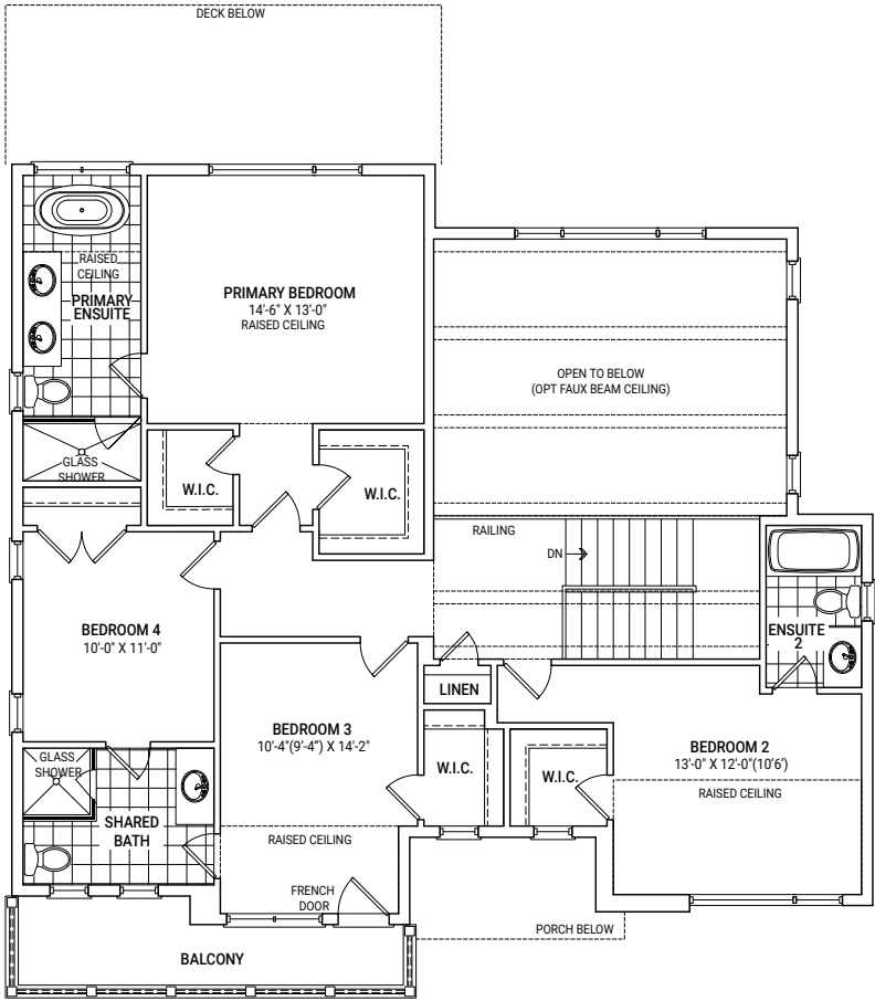
SECOND FLOOR PLAN ELEVATION D
