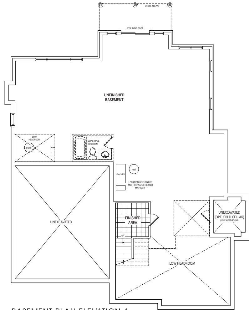
BASEMENT PLAN ELEVATION A
