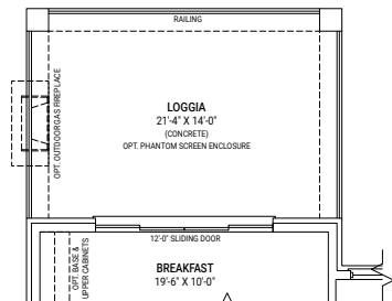
PARTIAL GROUND FLOOR PLAN ELE. A & D W/ OPT. LOGGIA
