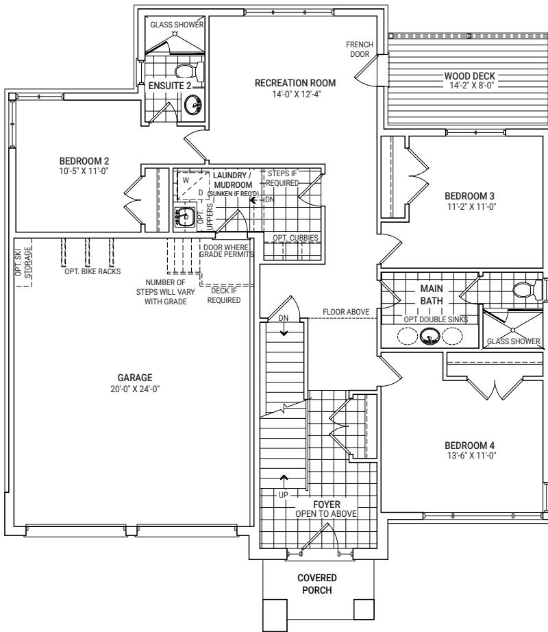
GROUND FLOOR PLAN ELEVATION A
