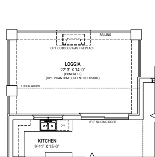
PARTIAL GROUND FLOOR PLAN ELEVATION A & D W/OPT. LOGGIA
