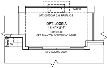
PARTIAL GROUND FLOOR PLAN ELEVATION A W/ OPT. LOGGIA
