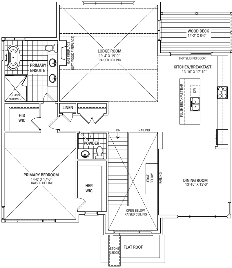
SECOND FLOOR PLAN ELEVATION A
