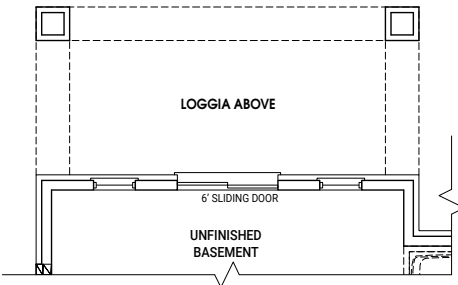
PARTIAL OPT. BASEMENT PLAN W/ OPT. LOGGIA
