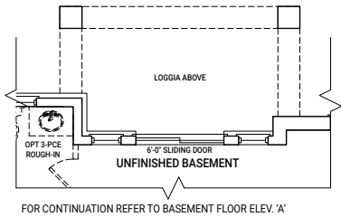
BASEMENT PLAN ELEVATION A W/ OPT. LOGGIA
