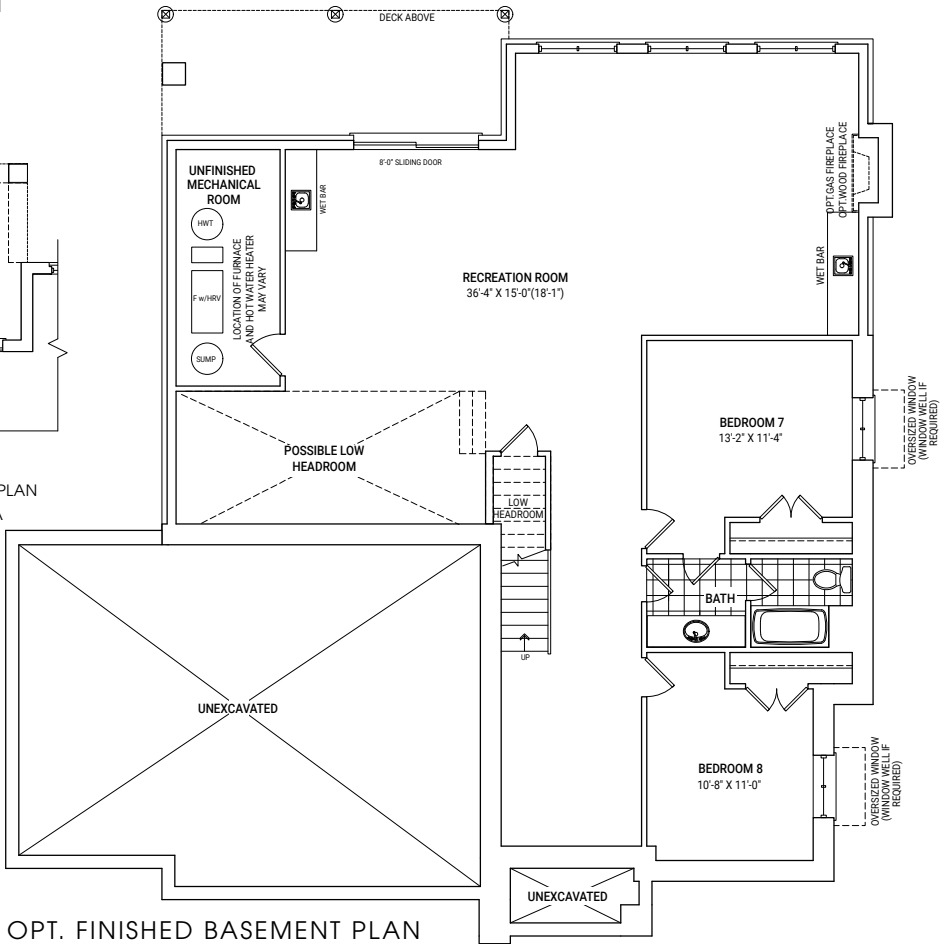
OPT. FINISHED BASEMENT PLAN ELEVATION A
