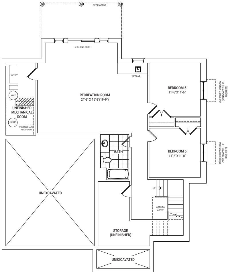
OPT. FINISHED BASEMENT PLAN ELEVATION B
