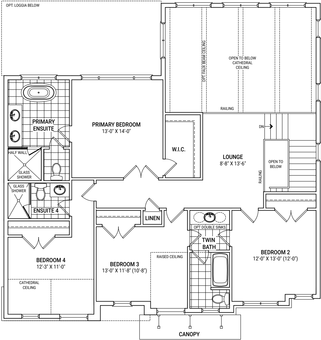
SECOND FLOOR PLAN ELEVATION D
