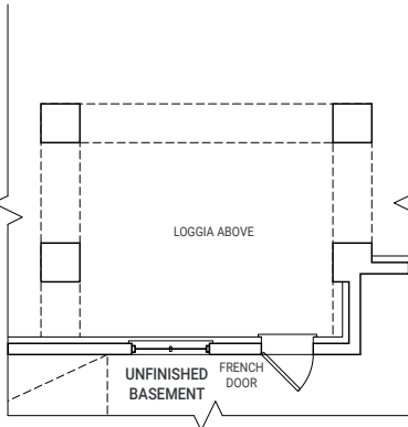
PARTIAL OPT. BASEMENT PLAN W/ OPT. LOGGIA
