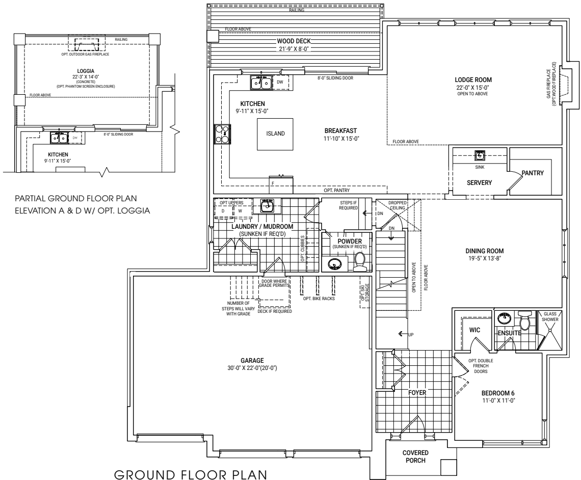
GROUND FLOOR PLAN ELEVATION A
