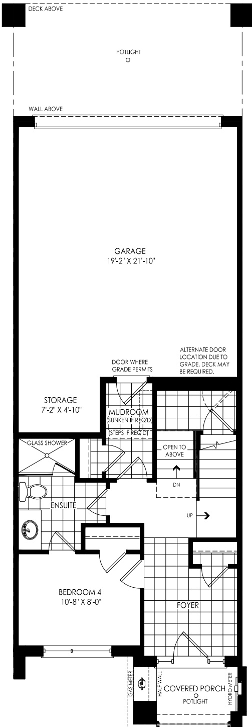
GROUND A2
