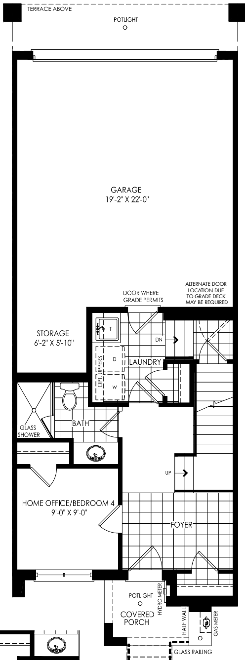
GROUND A
