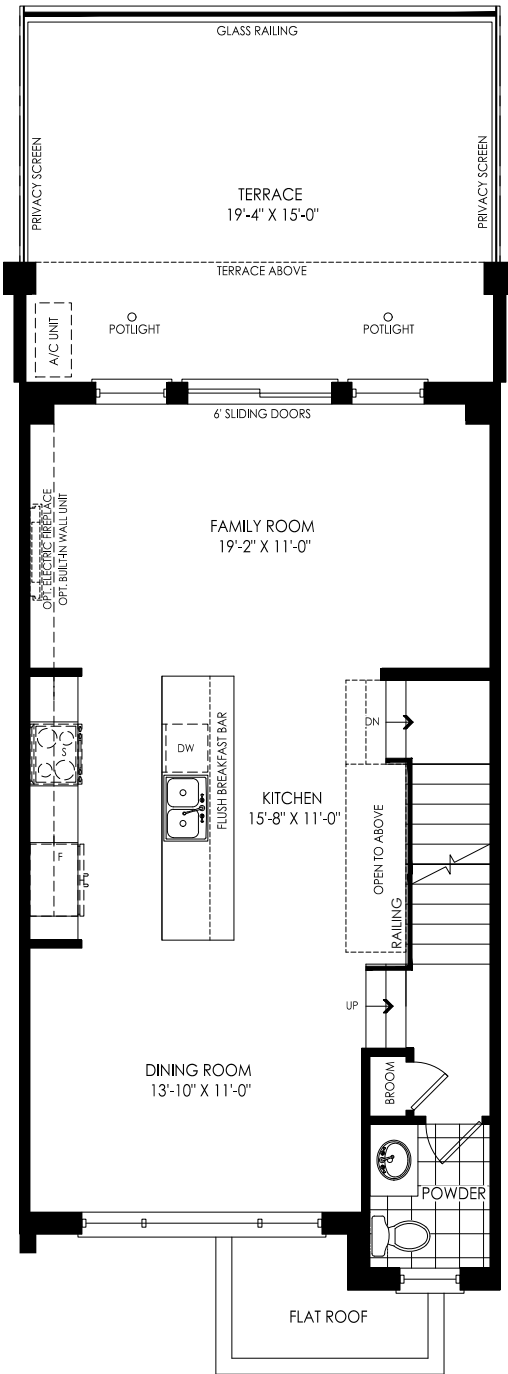
MAIN A
