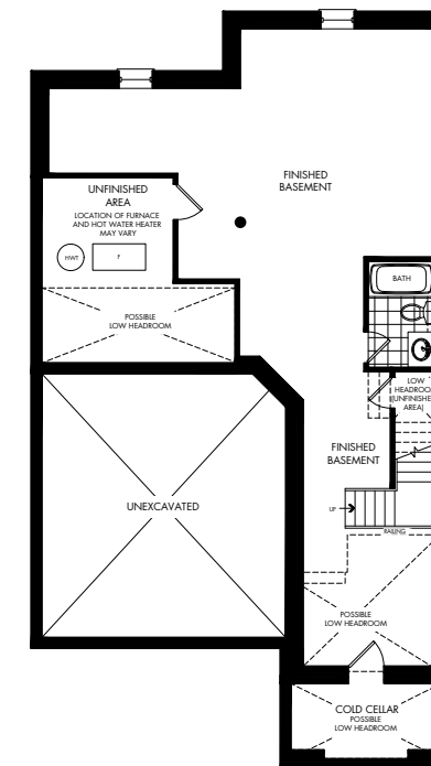
FINISHED BASEMENT A & B (OPTIONAL)
