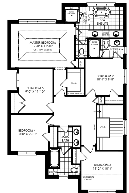
5 BED SECOND FLOOR A (OPTIONAL)
