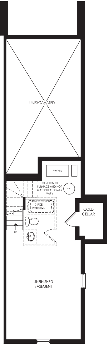
BASEMENT A
