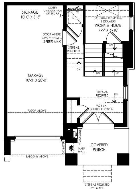
GROUND FLOOR ELEV. B (OPTIONAL 2 BATHROOM)
