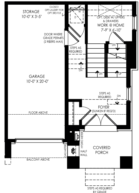
GROUND FLOOR ELEV. A (OPTIONAL 2 BATHROOM)
