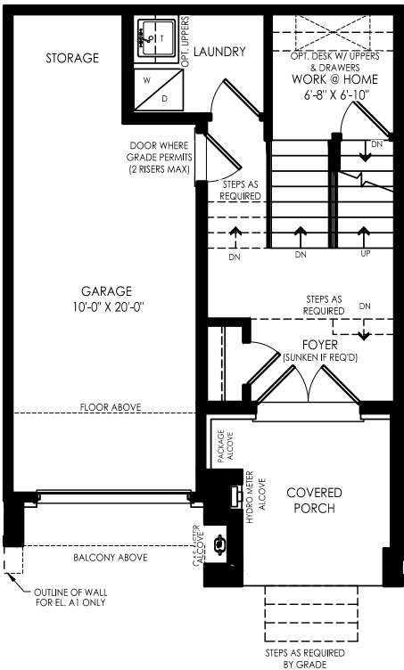
GROUND FLOOR ELEV. A
