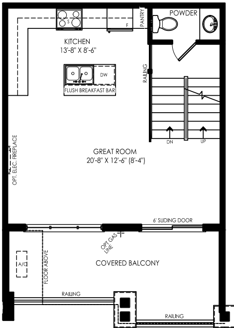
SECOND FLOOR ELEV. A
