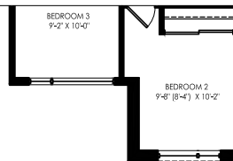
SECOND FLOOR ELEV. C
