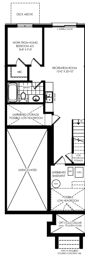
OPT. FINISHED WALK-OUT BASEMENT ELEV. A & B & C
