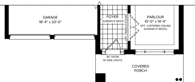
PARTIAL GROUND FLOOR ELEVATION C
