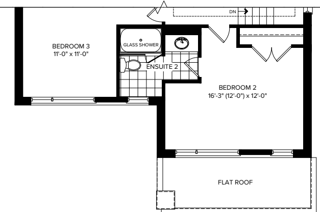
PARTIAL SECOND FLOOR ELEVATION C
