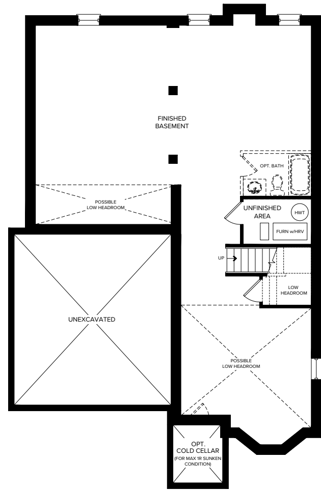
PARTIAL FINISHED BASEMENT ELEVATION B
