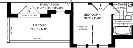
PARTIAL SECOND FLOOR ELEVATION B
