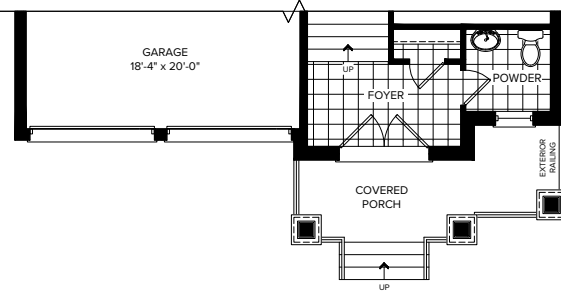
PARTIAL GROUND FLOOR ELEVATION B
