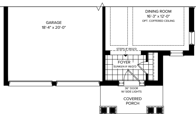
PARTIAL GROUND FLOOR ELEVATION B
