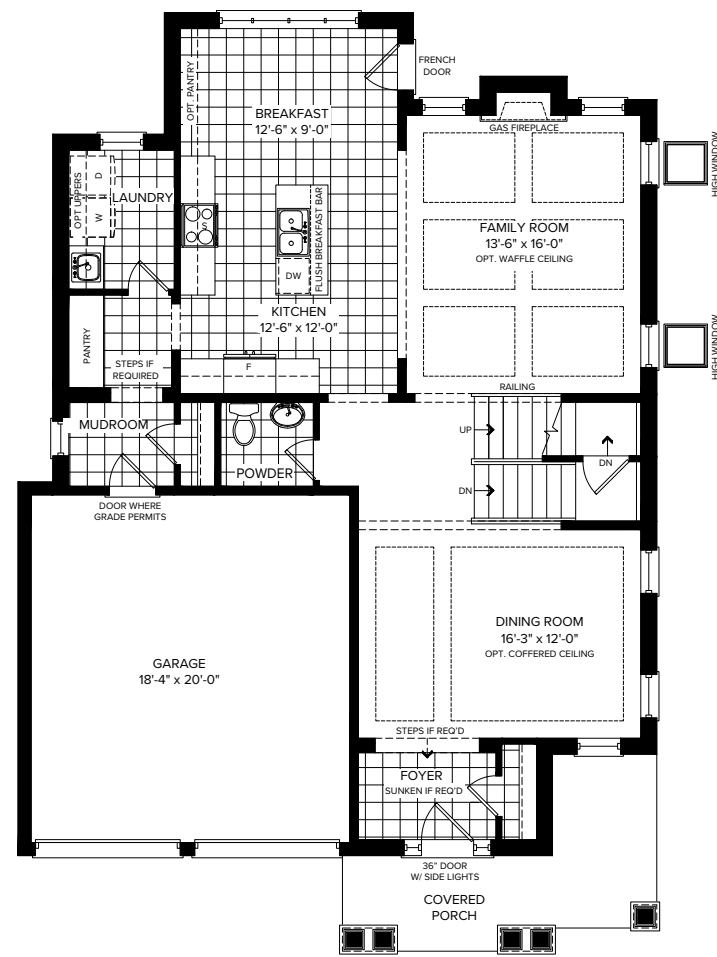
PARTIAL GROUND FLOOR ELEVATION B
