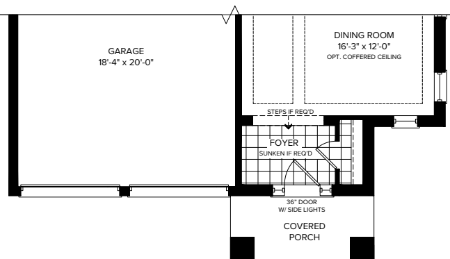
PARTIAL GROUND FLOOR ELEVATION C
