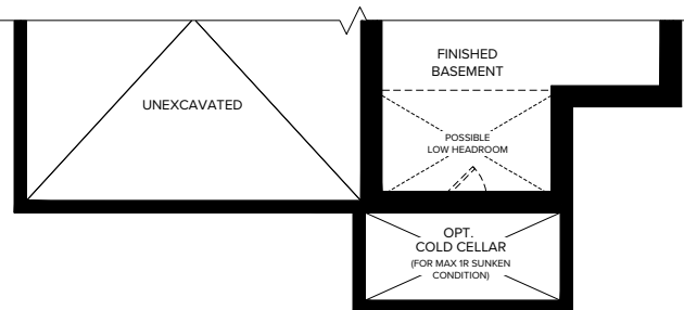
PARTIAL FINISHED BASEMENT ELEVATION B
