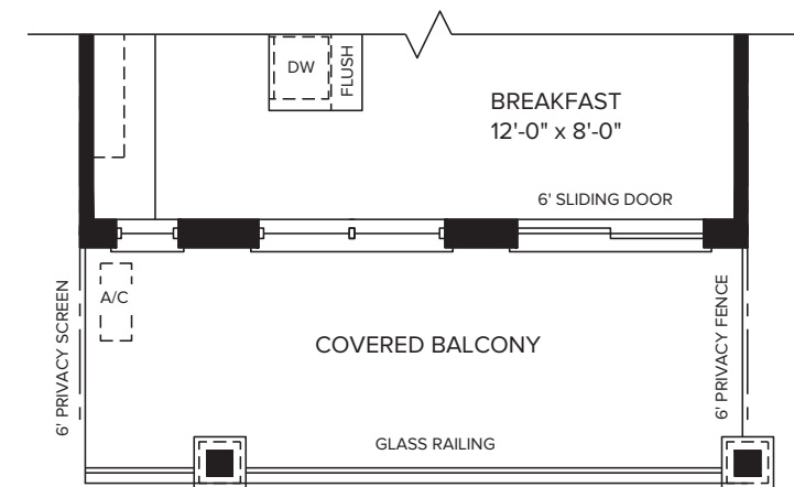
PARTIAL MAIN FLOOR ELEVATION B
