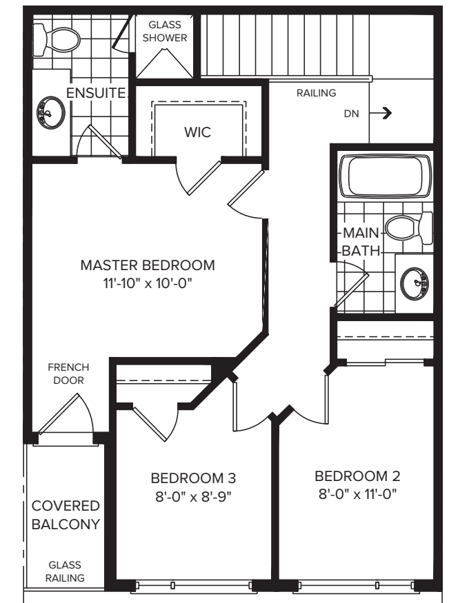
THIRD FLOOR ELEVATION A
